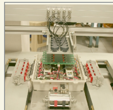
Testing bench for Composite Metering System
