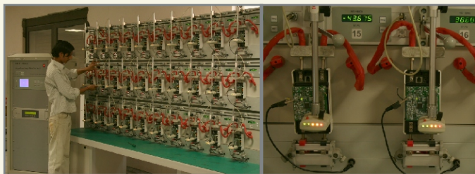
Meter Testing Bench
